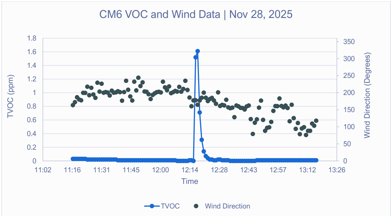
Figure 2 CM6 – Focus Points tVOC and Wind Direction November 28, 2025, 11:17 AM to 1:16 PM
