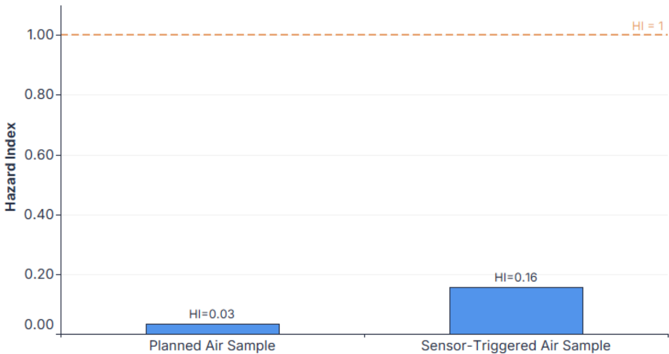
Figure 5 Hazard Indices at the CCND CM6 – Focus Points for Planned (December 9, 2025) and Sensor-Triggered (November 28, 2025) Air Samples
