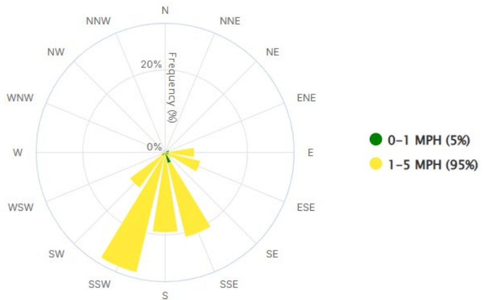
Figure 3 CM6 – Focus Points Wind Rose November 28, 2025, 11:17 AM to 1:16 PM
